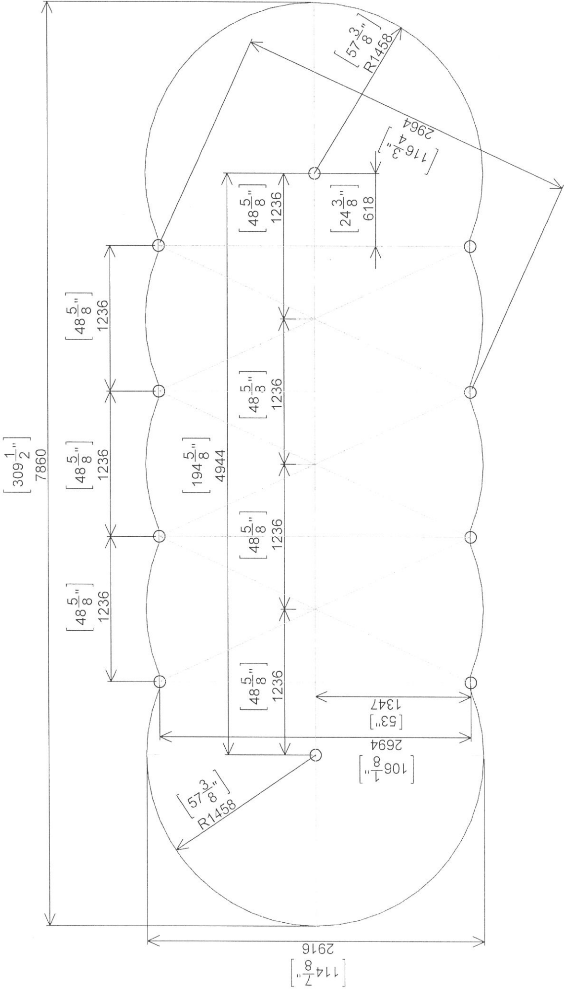
DRAWING POOL SHAPE 26x10
